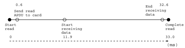
Figure 4: Breakdown of 8 byte read
