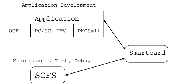
Figure 7: SCFS as a low-level development tool.
