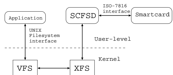
Figure 1: SCFS design
